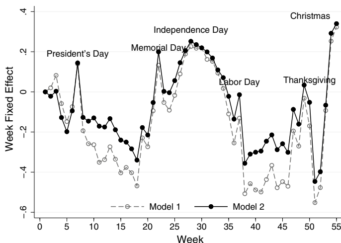
Fig. 2 Estimated seasonality
